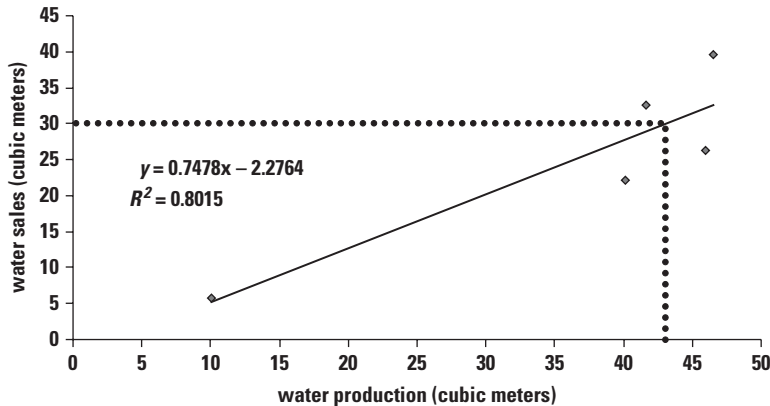
Figure A1.7 Relationship of Total Water Sales to Water Production for Utilities in Five Capital Cities
