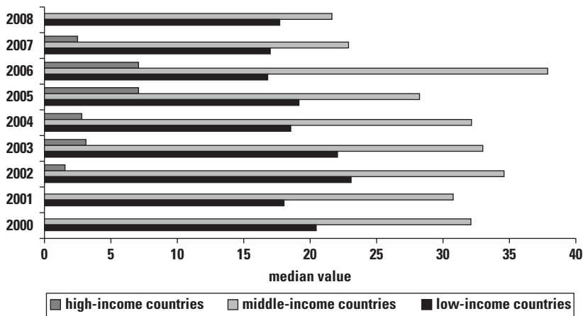
Figure 3.1 Nonrevenue Water (m 3 /km/day) by Income Level—Median Values
